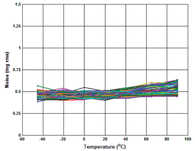
Figure 5.26 Accelerometer Noise over Temperature
