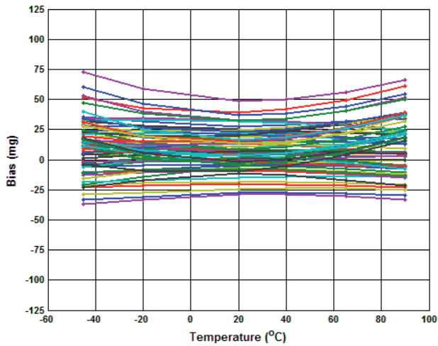
Figure 5.5 Accelerometer Bias
